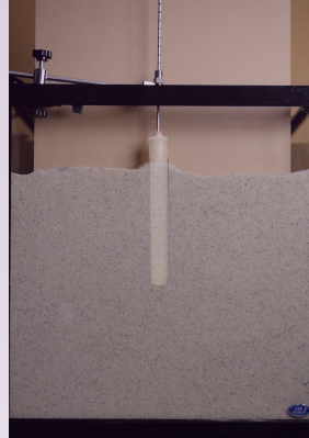
Self-burrowing robot
